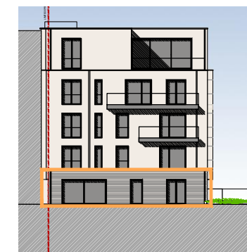
FACADE ARRIERE
